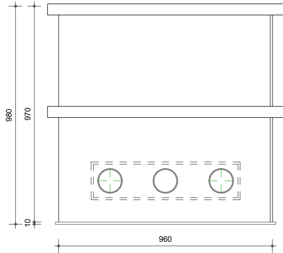
Front view
