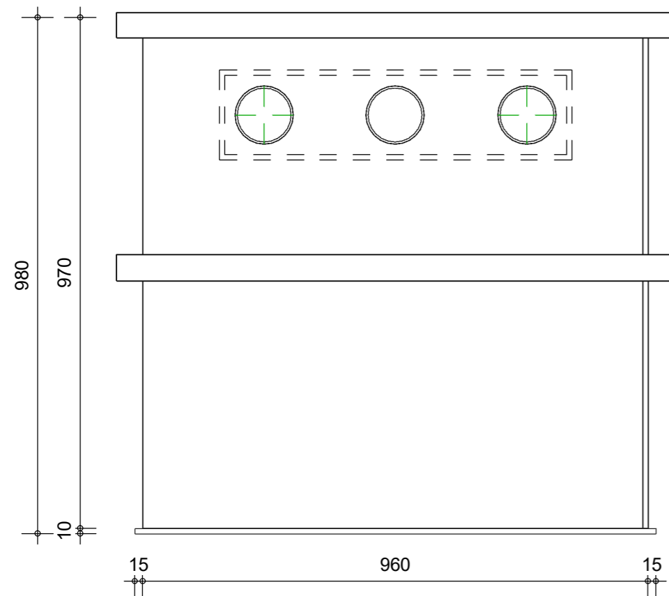
Rear view
